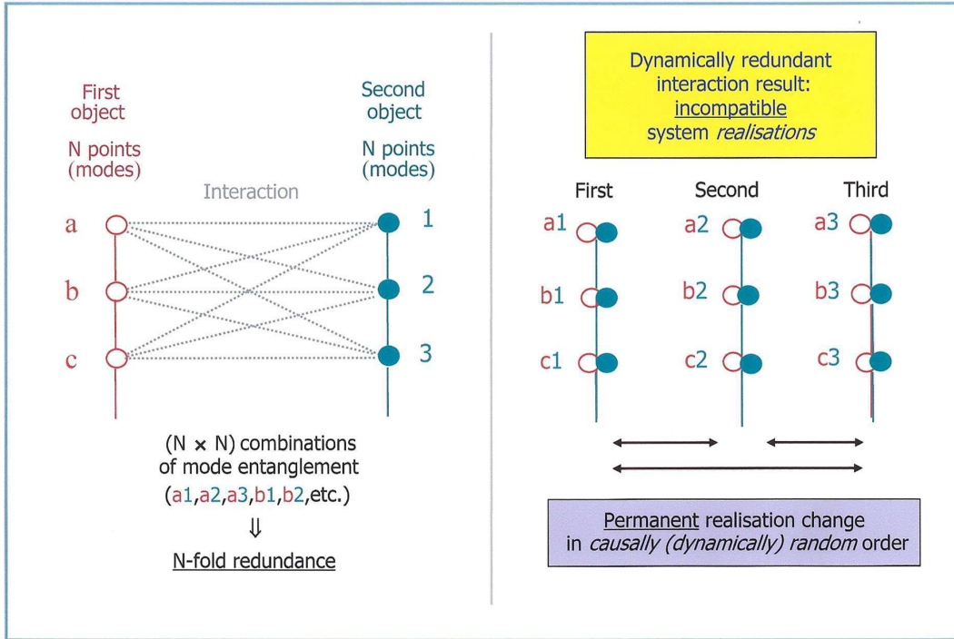
Figure 2. Dynamic multivaluedness emergence in any real interaction process. Unreduced interaction between two objects (e. g. protofields) with N interacting points or modes each (left) includes N^2 mode combinations, leading to N -fold redundance of incompatible system realisations thus formed (in agreement with equations (6), (11)). It is related to the symmetry of complexity , as the “number of places” for interaction components and products, determined by the total system complexity, cannot change in the course of interaction. Therefore all N_{\mathbb{R}} = N equally real system realisations are forced, by the same driving interaction, to permanently replace each other in a dynamically random order thus defined (right).
