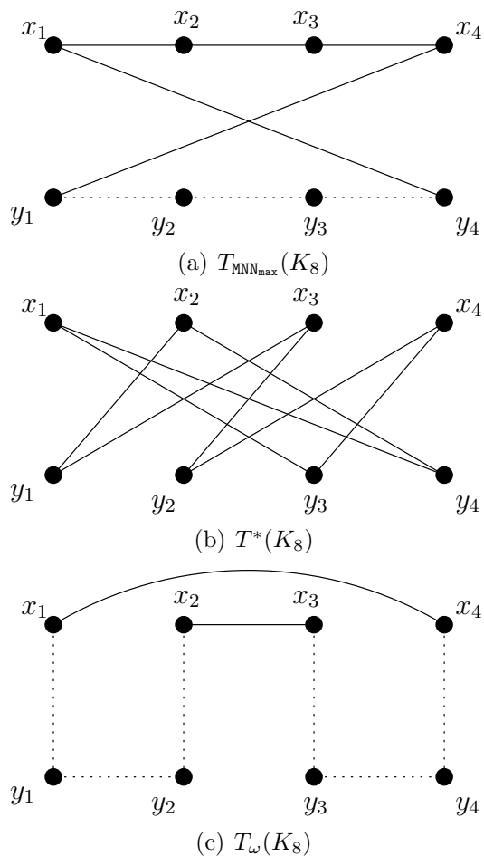
Figure 3: The tours T_{\text{MNN}_{\max}}(K_8) , T^*(K_8) and T_\omega(K_8) .
