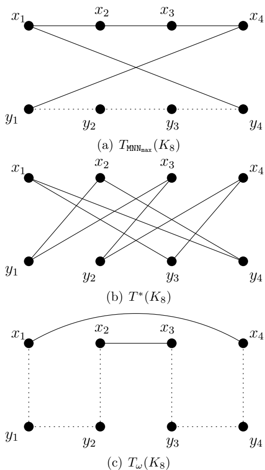
Figure 3: The tours T_{\text{MNN}_{\text{max}}}(K_8) , T^*(K_8) and T_\omega(K_8) .
