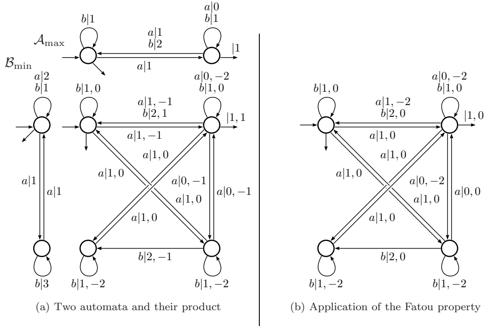
Figure 1: Getting an unambiguous automaton (I)
