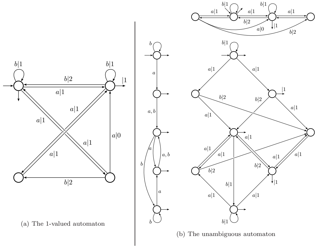
Figure 2: Getting an unambiguous automaton (II)
