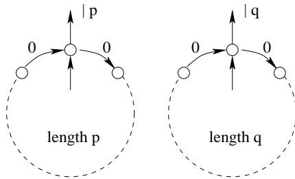
Figure 3: A max-plus automaton recognizing T_1 .
