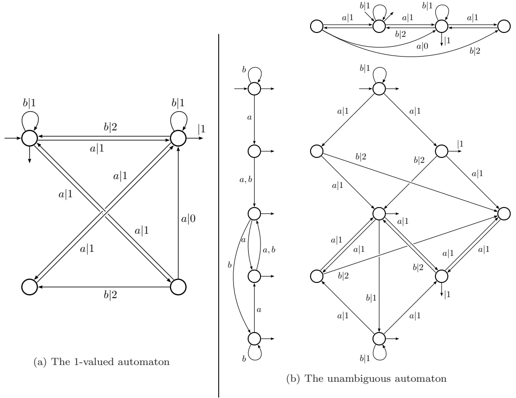
Figure 2: Getting an unambiguous automaton (II)
