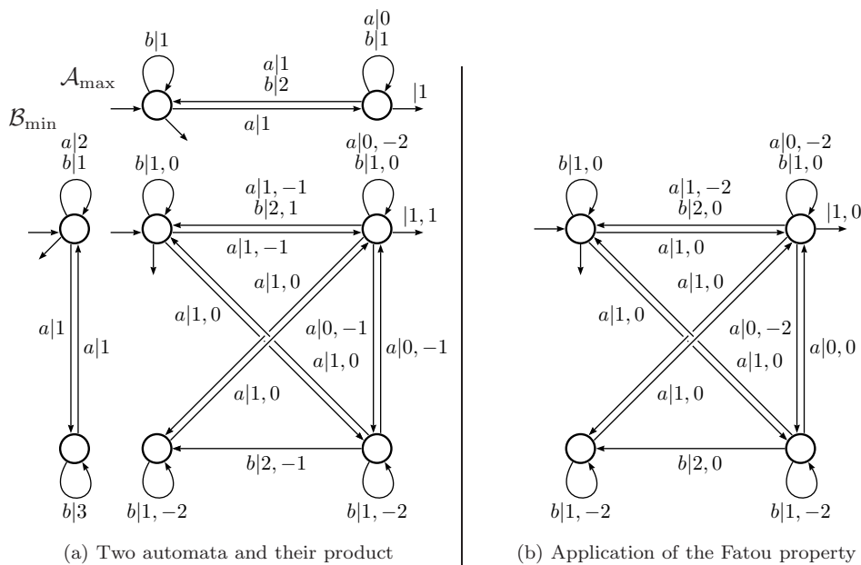
Figure 1: Getting an unambiguous automaton (I)
