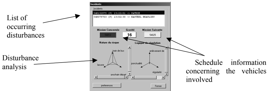
Figure 5: The regulator interface of the network incident management system
