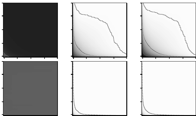
Fig. 14. AB graph: clustering, number of triangles, and number of triples. k = 10 , N = 10^4 , USP (first line) and ASP (second line).
