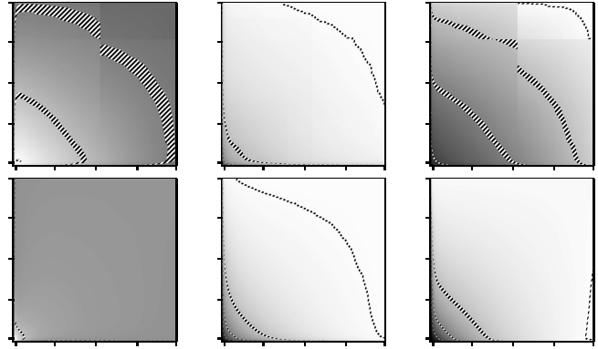
Fig. 17. Clustering, number of triangles, number of triples for the original Mercator graph (first line) and a GL graph with the same distribution of clique sizes (second line). USP explorations.
