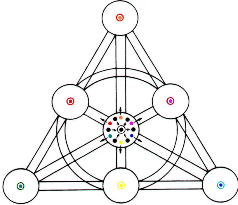
Figure 2: A schematic illustration of the properties of a homomorphism of \text{PR}_{\otimes}(2,2) into \text{PG}(2,2) on the behaviour of the neighbourhood (twelve small points in the central circle) of a point of \text{PR}_{\otimes}(2,2) (the big black doubled circle). The points of the associated (Fano) plane, \text{PG}(2,2) , are represented by seven big circles, six of its lines are drawn as pairs of line segments and the remaining line as a pair of concentric circles. As indicated by small arrows, the six points out of the twelve neighbours that are drawn black merge with the image of the reference point itself, while those six points drawn in different colours are sent in a one-to-one, colour-matching fashion into the remaining six points (the big coloured doubled circles) of \text{PG}(2,2) .
