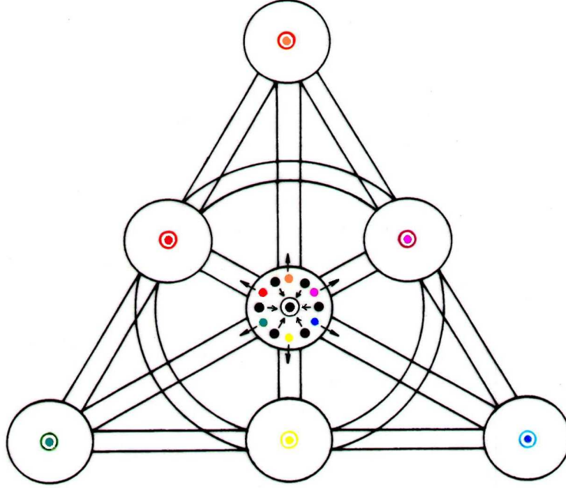
Figure 1: A schematic illustration of the properties of a homomorphism of \text{PR}_{\otimes}(2,2) into \text{PG}(2,2) on the behaviour of the neighbourhood (twelve small points in the central circle) of a point of \text{PR}_{\otimes}(2,2) (the big black doubled circle). The points of the associated (Fano) plane, \text{PG}(2,2) , are represented by seven big circles, six of its lines are drawn as pairs of line segments and the remaining line as a pair of concentric circles. As indicated by small arrows, the six points out of the twelve neighbours that are drawn black merge with the image of the reference point itself, while those six points drawn in different colours are sent in a one-to-one, colour-matching fashion into the remaining six points (the big coloured doubled circles) of \text{PG}(2,2) .
