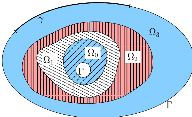
Figure 7: A geometrical situation for which only on set of weight functions is need to obtain a Carleman estimate.
