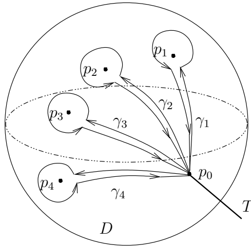
FIGURE 6. Holonomie projective
