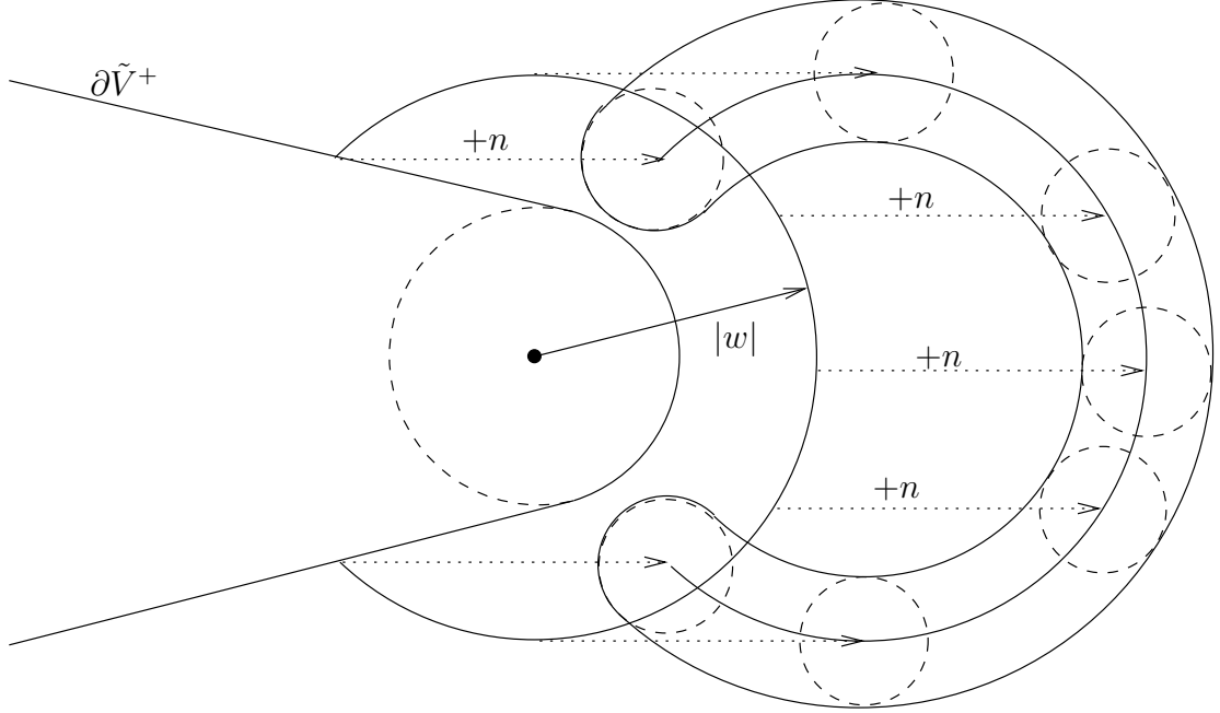
FIGURE 4. Minimiser \frac{|\tilde{f}^{o n}(w)|}{(|w|+n)}
