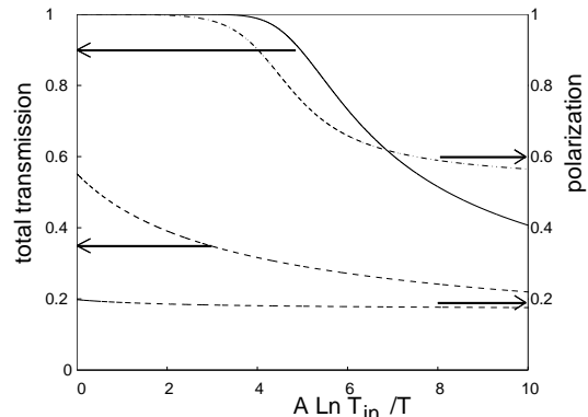
FIG. 3: Total transmission and polarization as a function of the logarithm of the temperature. The two curves marked with left arrows represent the total transmission for \Gamma = 1.01 (solid line) and \Gamma = 10 (dashed line). The two other curves represent the spin polarization for \Gamma = 1.01 (dash-dotted line) and \Gamma = 10 . (dashed line) respectively.
