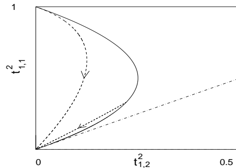
FIG. 2: Solid line: location of the initial points. Upper dashed line: renormalization group flow for \Gamma = 1 . The starting point is at t_{1,1} = 1 . Lower dashed line: renormalization group trajectory for \Gamma = 10 . The dashed-dotted line is simply the first diagonal, corresponding to totally unpolarized beams and reaches t_{1,1}^2 = 1 at t_{1,2}^2 = 1 .
