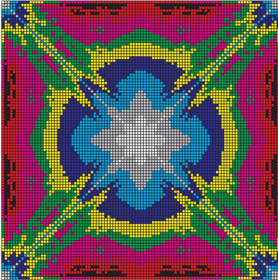
FIGURE 4. Number of topplings to compute the identity on the 100 \times 100 grid. From white (less than 10) to black (more than 80).
