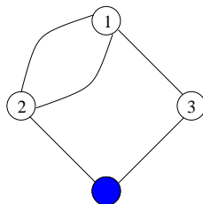
FIGURE 1. Multigraph with 4 vertices
