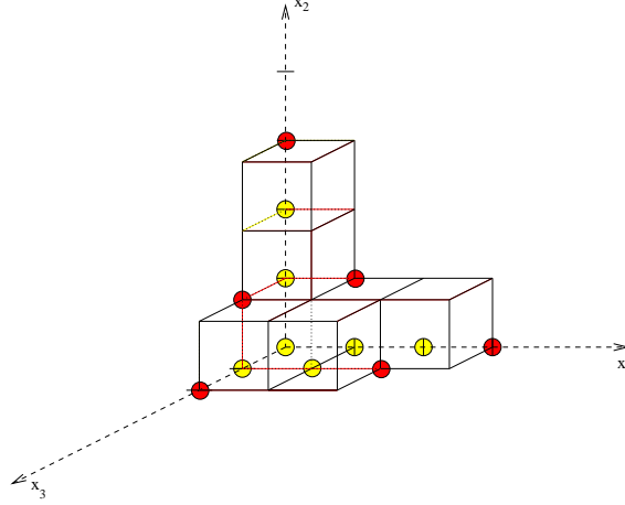
FIGURE 2. Staircase of the Gröbner basis
