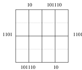
FIGURE 2. A quasi-tiling (also a tiling)
