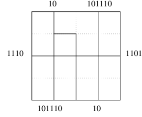
FIGURE 3. A quasi-tiling
