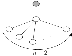
Figure 11: Tree T_n .
