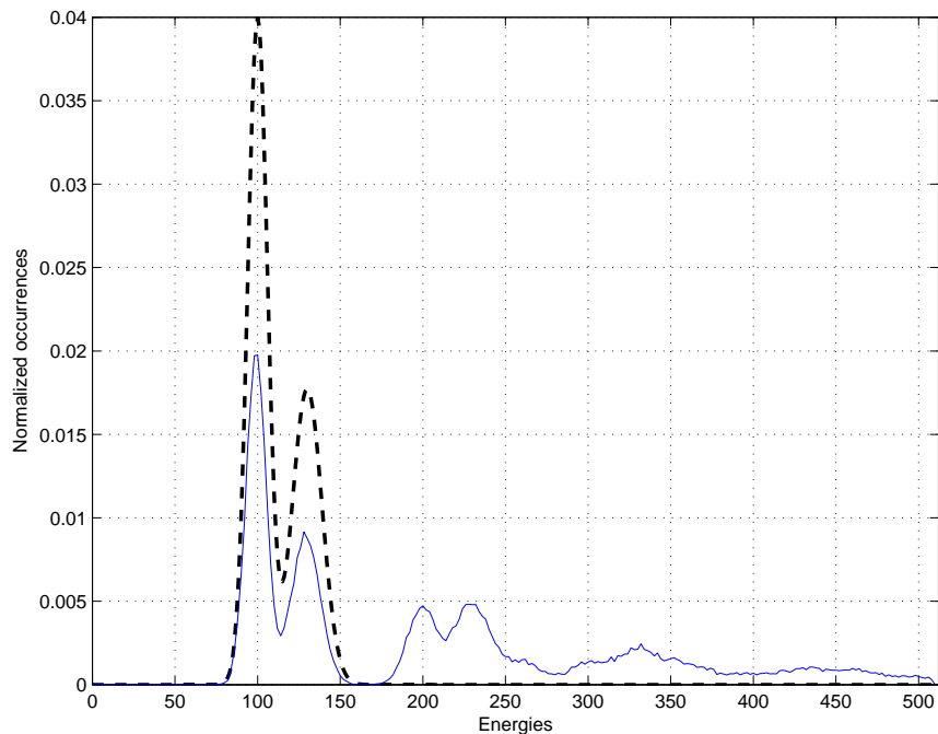
FIGURE 2. dashed line: marginal density of the energy for the pdf (44); solide line: kernel density estimator of the pileup observations based on 10^5 samples.
