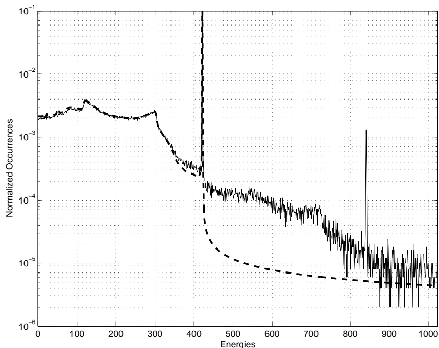
FIGURE 4. Illustration of ideal and piled-up energy spectra of the Cs 137 element
