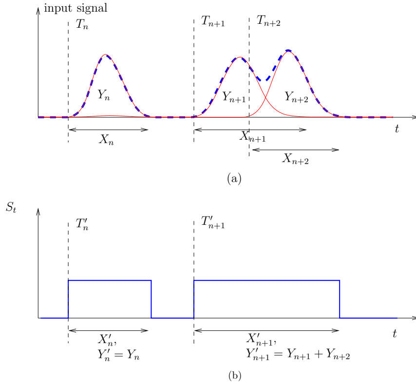
FIGURE 1. Illustration of the pile-up phenomenon. (a) : input signal with arrival times T_j , lengths X_j and energies Y_j , j = n, \dots, n + 2 ; (b) : associated on-off process S_t , S_t = 1 if the system is busy at time t and S_t = 0 otherwise.
