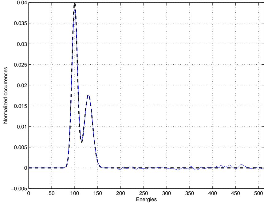
FIGURE 3. dashed line: marginal density of the energy for the pdf (44); solid line: estimator \hat{m}_{x,h,n} .
