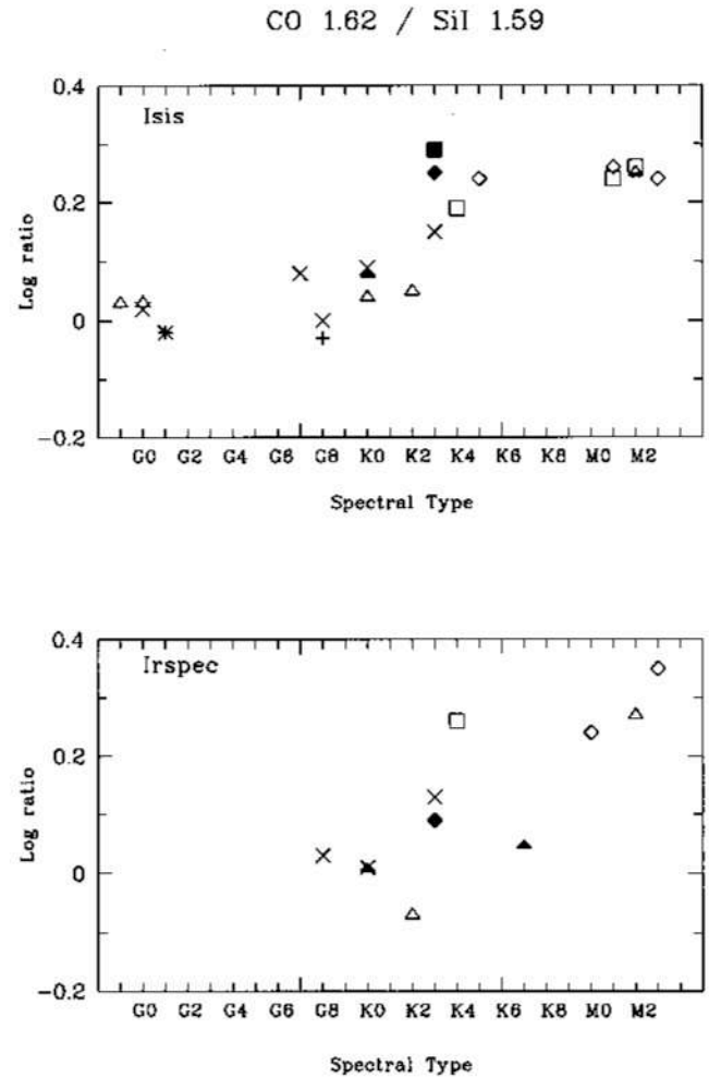
Fig. 7. Variations of the line ratio, (\text{CO}+\text{CaI})\lambda 1.62 \mu\text{m} over \text{SiI}\lambda 1.59 \mu\text{m} , with spectral type and luminosity class. Same symbols as in Fig. 4
