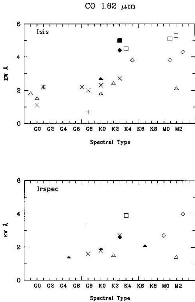
Fig. 6. Variations of CO 1.62 \mu\text{m} with spectral type and luminosity class. Same symbols as in Fig. 4
