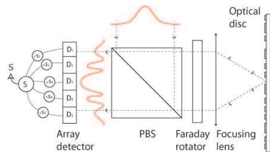
FIG. 1: Color online Scheme for information extraction from optical disc, using an array detector.
