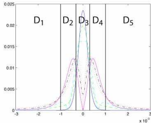
FIG. 8: Color online Far field profiles in detection the plane for each bit configuration, and array detector geometry. The 5 detectors D_1..D_5 have electronic gains \sigma_1(i).. \sigma_5(i) according to the bit sequence i which is present in the focal spot.
