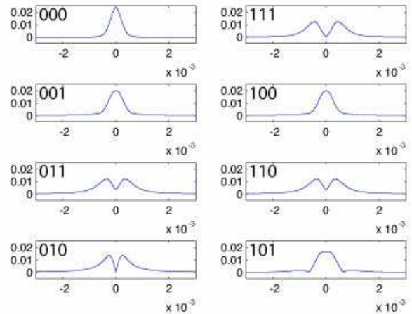
FIG. 6: Color online Field profiles in the array detector plane, for each of the 8 bit sequence configuration. Note that they are clearly distinguishable, except for the bit sequences 100 and 001, and 011 and 110, which have the same profile because of the symmetry of the bit sequence relative to the position of the incident laser beam.
