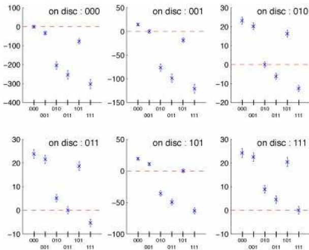
FIG. 11: Color online Quantum detection noise represented as error bars, for \lambda = 0.78\mu\text{m} , NA = 0.47 , 25 detected photons and -10\text{ dB} of simultaneous squeezing for all the flipped modes. The ambiguity in presence of shot noise has been removed and each bit sequence can be identified.
