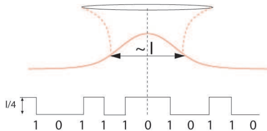
FIG. 2: Color online Example of bit sequence on an optical disc. The spacing between the bits is smaller than the wavelength, the minimum waist of the incident laser beam being of the order of \lambda . A hole depth of \lambda/4 insures a \pi phase shift between fields reflected on a pit and a hole.
