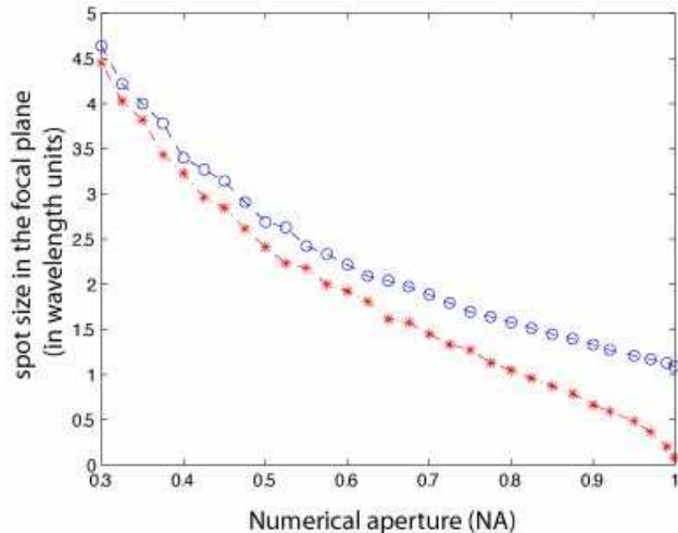
FIG. 3: Evolution of the focused spot size of an incident plane wave with the numerical aperture (for \lambda = 780 nm in air medium). The spot size is limited to the order of the wavelength in the non-paraxial case (o), whereas it goes to zero for very high numerical apertures in the paraxial case(*).
