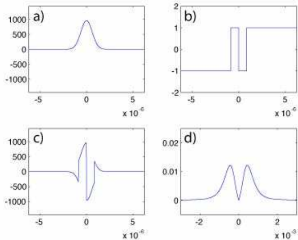
FIG. 5: Color online Modifications of the transverse amplitude field profile through propagation, in the case of a 111 bit sequence in the focal spot : a) incoming beam profile, b) 111 bit sequence, c) corresponding reflected field in the disc plane, d) far field profile in the detector plane .
