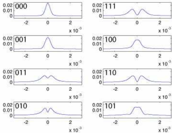
FIG. 7: Color online Far field profiles in the array detector plane, for each of the 8 bit sequence configuration, when the position of the disc has been shifted of w_0/6 relative to the incident beam. The profile degeneracy for 100 and 001, and 011 and 110 is raised. Note that the other profiles have experienced a much smaller shape modification between the two positions of the disc.
