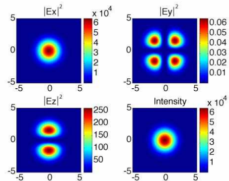
FIG. 4: Color onlineNorm of the different field components and resultant intensity in the focal plane with a linearly polarized incident field along the x axis, focused with a 0.47 numerical aperture.
