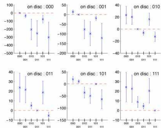
FIG. 9: Classical noise (10 dB of excess noise) represented as error bars, for \lambda = 0.78\mu m , NA = 0.47 , and 25 detected photons. Each inset corresponds to the 6 signals obtained for the different gain configurations, when one particular bit sequence is present in the focal spot. Each bit sequence present in the focal spot can be clearly identified as only one gain configuration can give a zero value for each inset.
