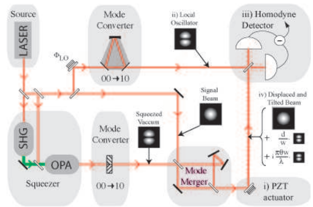
FIG. 1: Schematic diagram of the experiment for optimal displacement and tilt measurements with a spatial homodyne detector. A TEM_{00} mode, which is displaced and tilted using a PZT actuator (i), is mode-matched to the TEM_{10} local oscillator (ii) of a balanced homodyne detector (iii). The TEM_{10} local oscillator selects the quadratures amplitude of the TEM_{10} component of the input beam that contains the small displacement and tilt information of the incident TEM_{00} beam (iv).
