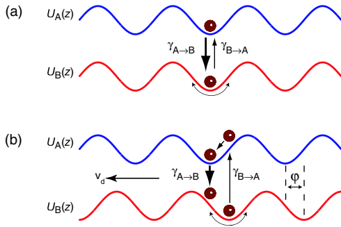
FIG. 1 (color online). Rectification mechanism. Atoms move in two symmetric potentials U_A(z) and U_B(z) that are coupled via the asymmetric optical pumping rates \gamma_{A \rightarrow B} and \gamma_{B \rightarrow A} ( \gamma_{A \rightarrow B} \gg \gamma_{B \rightarrow A} ). (a) The potentials are in phase. The transfer from the long-lived state B, to the transient state A, and back, does not lead to biased motion. (b) A phase shift \varphi is introduced. Spatial diffusion is strongly facilitated in one direction, leading to a drift velocity v_d .
