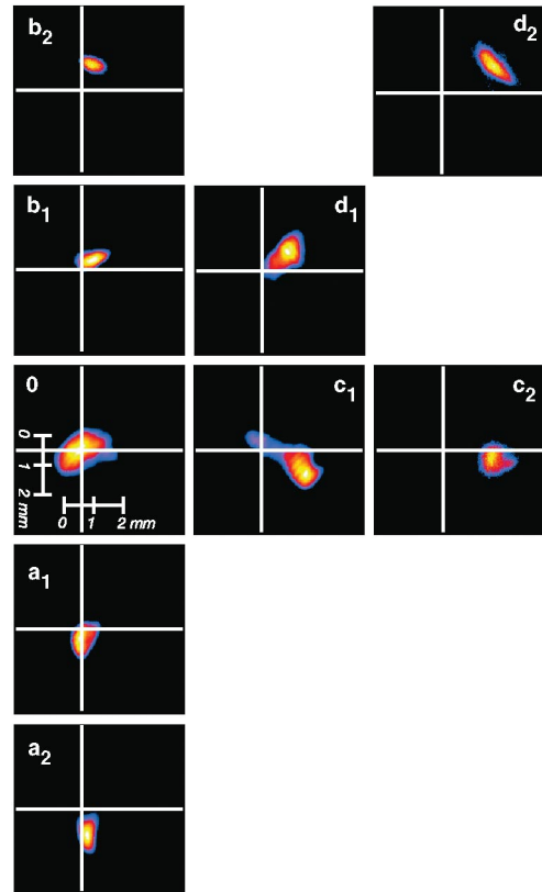
FIG. 3 (color). Images of the atomic cloud. The image labeled “0” shows the initial cloud. The series labeled “a 1 -a 2 ” are images taken at two different interaction times (0.4 and 0.9 s, respectively) for a phase shift along z . For images “b 1 -b 2 ,” the phase shift is still along z , but differ by \pi . The series “c 1 -c 2 ” is obtained when the phase shift is along x . Finally, a diagonal drift is displayed in “d 1 -d 2 ,” where the phase is shifted both along z and along x .
