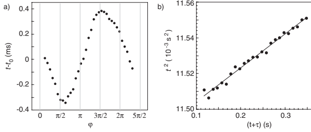
FIG. 2. (a) Induced directed drift in the vertical ( z ) direction, measured as arrival time t at a probe beam as a function of the relative spatial phase \varphi for an interaction time \tau of 350 ms. t_0 is the arrival time for zero drift velocity. (b) Confirmation of a constant drift velocity obtained by plotting t^2 as a function of t + \tau for different \tau . The line is a linear fit.
