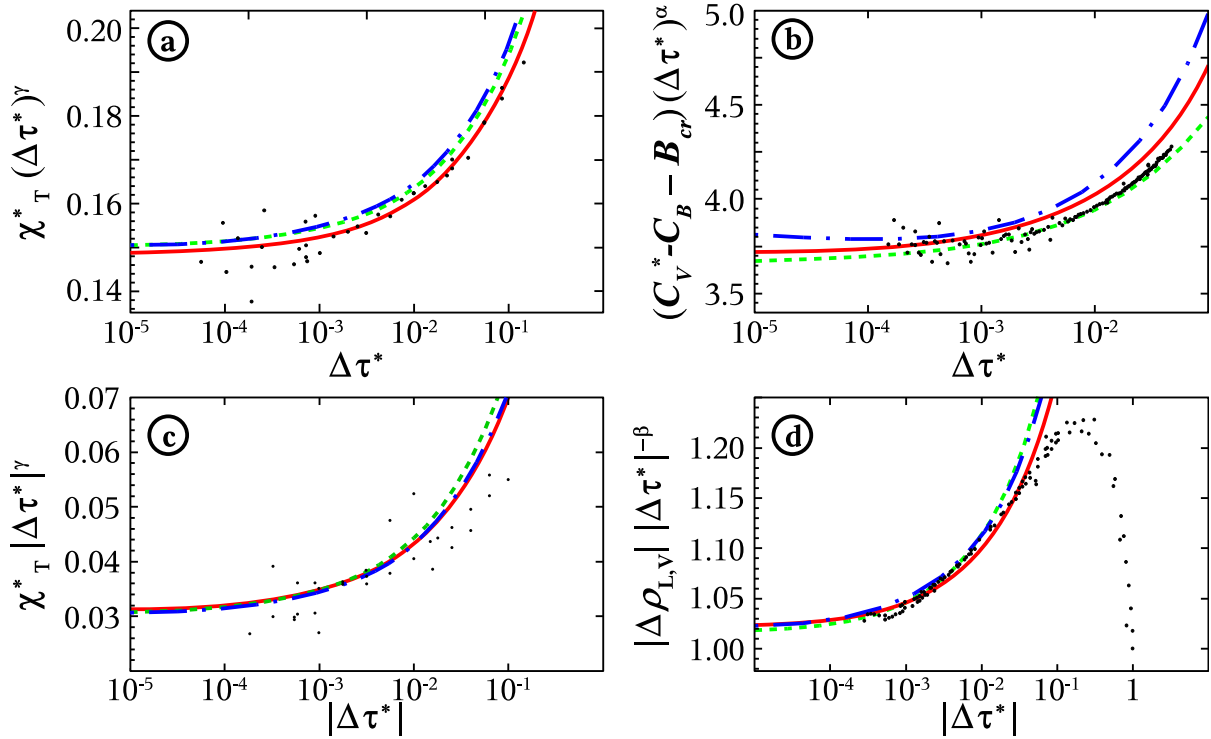
Figure 1: Asymptotic two-term predictions compared to the ^3\text{He} measurements (black points). The solid (red) lines are the actual predictions by the dilated scale method (see Eq. (24) and column 4 of Table II). The dot-dashed (blue) lines are the two-term prediction obtained from the best fit by the MSR \Phi_{d=3}^4(1) -model [14] (Eq. (24); column 2 of Table II). The dashed (green) lines are the two-term prediction obtained from CPM model [36] (Eq. (24); column 3 of Table II). (a) Susceptibility measurements for T > T_c (corresponding to upper part of Fig. 1 in [14]). (b) Specific heat measurements for T > T_c , where the small difference in the additional constant term C_B + B_{cr} is accounted in the vertical scale (see also the lower part of Fig. 3 in [14]). (c) Susceptibility measurements for T < T_c (see also the lower part of Fig. 1 in [14]). (d) Liquid-gas coexisting density measurements (see also Fig. 4 in [14]).
