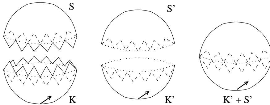
Figure 2: Gluing two quadrangulations with simple boundary.
