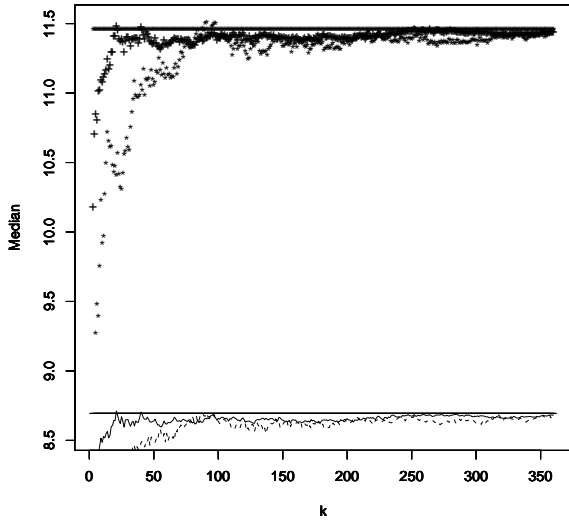
(a) Median as a function of k_n
