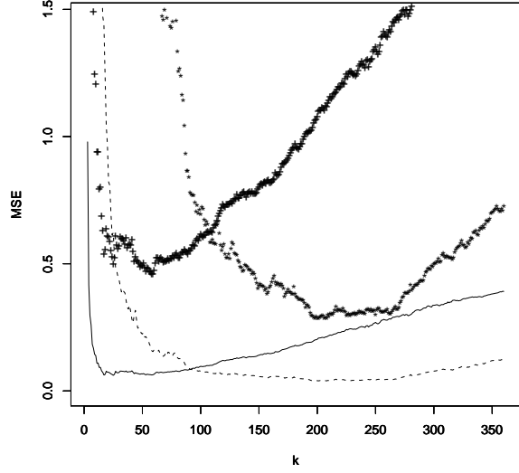
(b) MSE as a function of k_n
