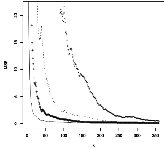
(b) MSE as a function of k_n
