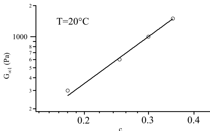
Figure 7: Plateau modulus G_{\infty 1} of the slow relaxation mode in the C_{12}EO_6/H_2O system at 20^\circ C as a function of the concentration. The line is a power-law fit with exponent 2.6.
