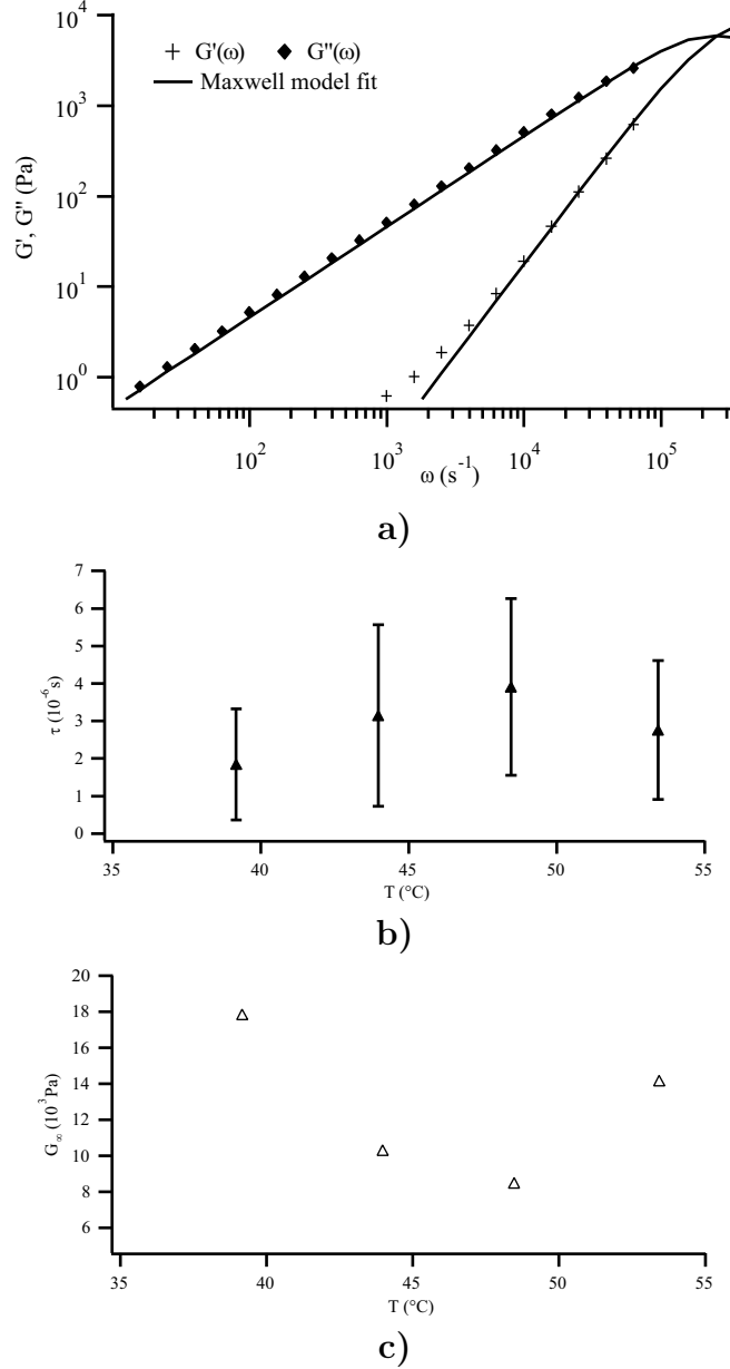
Figure 6: Rheology results for the C_{12}EO_8/D_2O mixture at c = 30\% : a) Maxwell model fit at T = 48.5^\circ C b) relaxation time \tau and c) plateau modulus G_\infty as a function of temperature.
