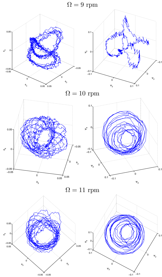
Figure 7: Left column: projection of u(\theta, t) on (\phi_2, \phi_3, \phi_4) for \Omega = 9, 10, 11 rpm. Right column: projection of u(\theta, t) on (\psi_2, \psi_3, \psi_4) for \Omega = 9, 10, 11 rpm.
