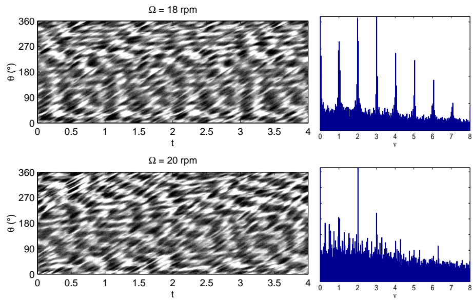
Figure 5: Space-time diagrams on the circle r = 0.7R , for higher values of the angular velocity \Omega (18 and 20 rpm), for which coherent structures are not anymore recognizable (time is expressed in number of rotations and \theta is the azimuthal angle). We also show the corresponding temporal Fourier spectra averaged on \theta .
