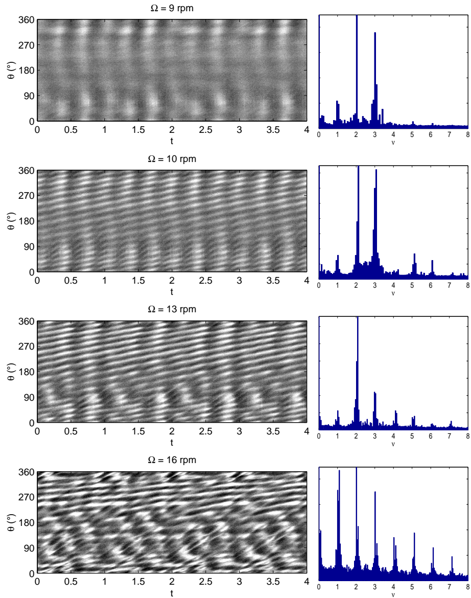
Figure 4: Windows of space-time diagrams on the circle r = 0.7 R , for some typical values of the angular velocity \Omega and for a duration of 4 disk rotations. We also show in arbitrary linear scale, the corresponding temporal Fourier spectra averaged on \theta .
