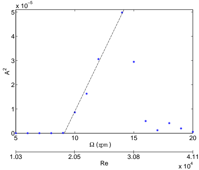
Figure 3: Squared amplitude of the grey level fluctuations corresponding to the spiral waves versus \Omega ; the typical linear behavior corresponding to the Hopf bifurcation is recovered.
