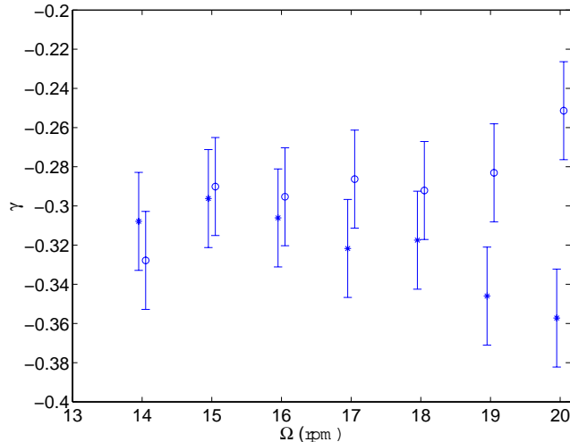
Figure 12: Azimuthal group velocity of the wave packets versus rotation rate \Omega . (*) central wave packet, ( \circ ) side wave packets. The central packet is entrained with the mean azimuthal velocity of the turbulent flow (between 0.3 and 0.4\Omega ).
