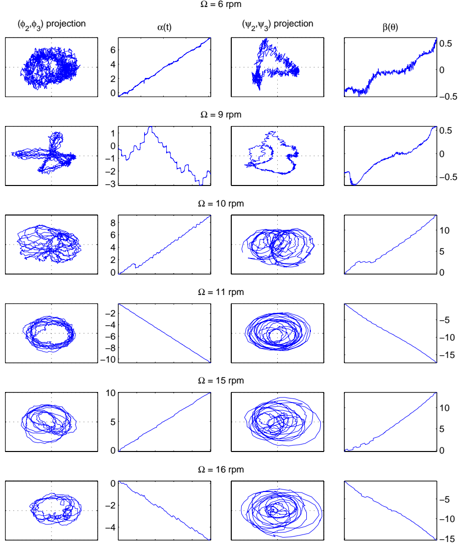
Figure 6: Left column: projection of u(\theta, t) on (\phi_2, \phi_3) for typical values of \Omega (the horizontal and vertical axis correspond to a fixed interval [-0.07, 0.07] ). Second column: angle \alpha(t) (in units of 2\pi ) between the horizontal axis \phi_2 and \xi_t^{2,3} , as a function of time during 5 disk rotations. Third column: projection of u(\theta, t) on (\psi_2, \psi_3) (the horizontal and vertical axis correspond to a fixed interval [-0.13, 0.13] ). Fourth column: angle \beta(\theta) (in units of 2\pi ) between the horizontal axis \psi_2 and \eta_\theta^{2,3} , as a function of \theta .
