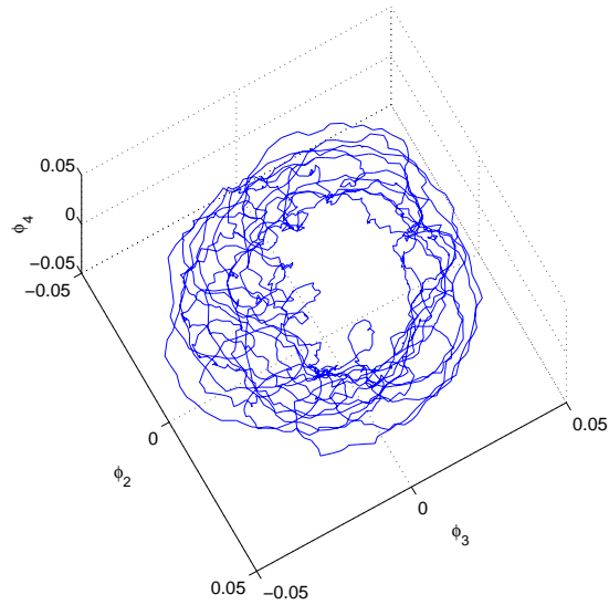
Figure 10: Projection of u(\theta, t) on (\phi_2, \phi_3, \phi_4) for \Omega = 16 rpm. The trajectory mainly winds up around the torus but small loops escaping from this torus are visible.
