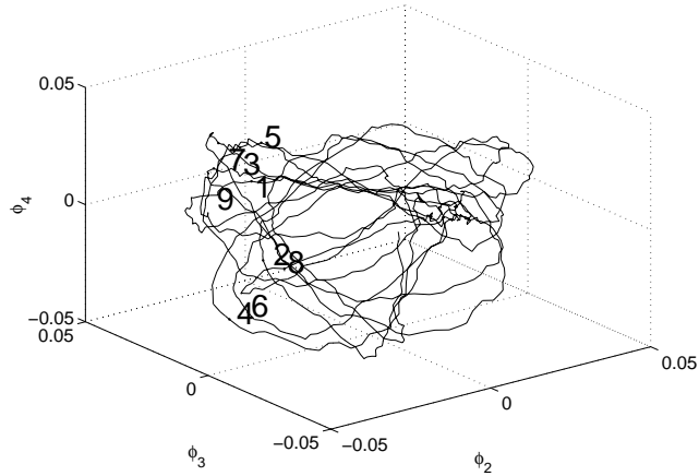
Figure 9: Projection of u(\theta, t) on (\phi_2, \phi_3, \phi_4) for \Omega = 15 rpm. In the picture, we labelled the points of the orbit separated by a same time delay equal to the period T of the dynamics on the torus before the bifurcation. The separation between odd and even loops is clearly visible: the torus doubling bifurcation just happened.
