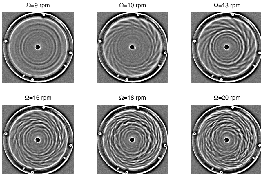
Figure 2: Images of the flow for some values of \Omega , the angular velocity of the disk. Clockwise rotation.
