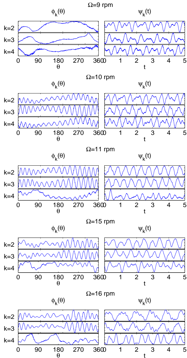
Figure 8: Plot of the first three topological modes and their corresponding chronos for \Omega = 9, 10, 11, 15, 16 rpm.
