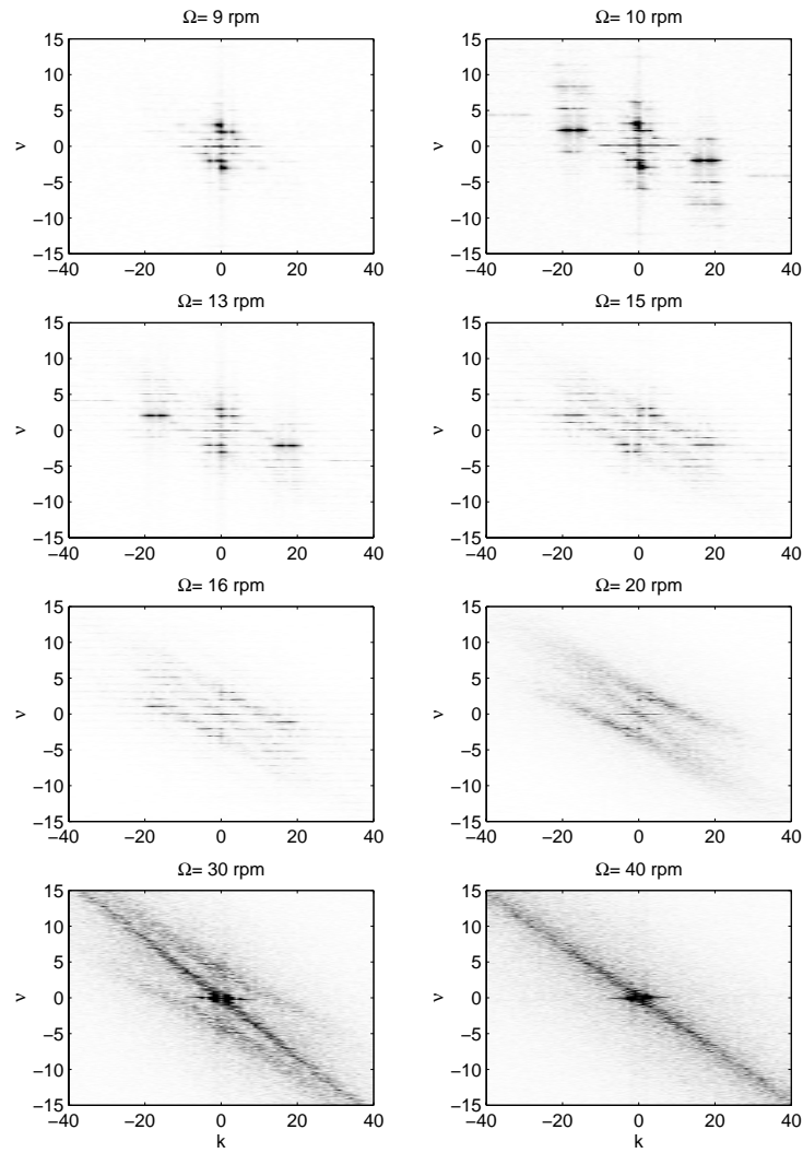
Figure 11: 2D-Fourier spectra of space-time diagrams for \Omega = 9 to 40 rpm.
