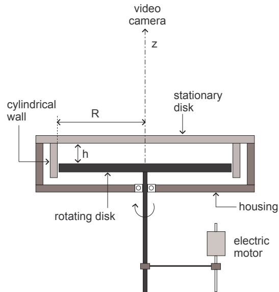
Figure 1: Experimental device.
