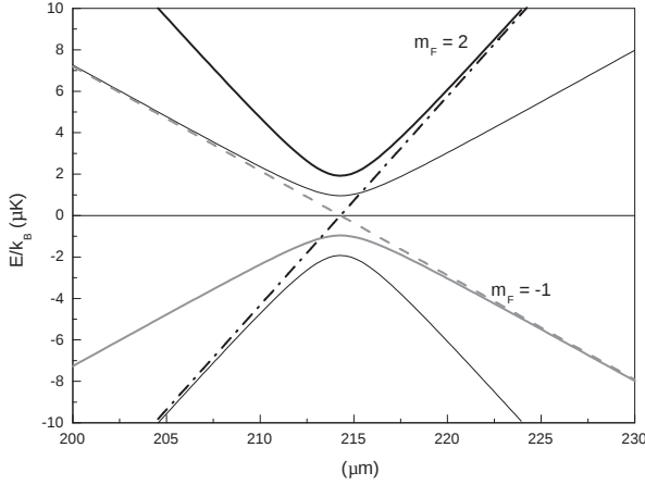
FIG. 1: Energy of the dressed levels in the magnetic quadrupole trap described in the paper, plotted along the radial coordinate, in the vicinity of the potential minimum at \rho = r_0 . The five dressed sub levels for a F = 2 spin state are plotted, as well as two bare states for comparison (bare state m_F = -1 is shown dashed and m_F = 2 dash-dotted). The ring trap we discuss in this paper is based on the upper dressed potential m_F = F = 2 , for the radial trapping (bold solid line). Values for the field gradient, and rf and Rabi frequencies are given in Table I.
