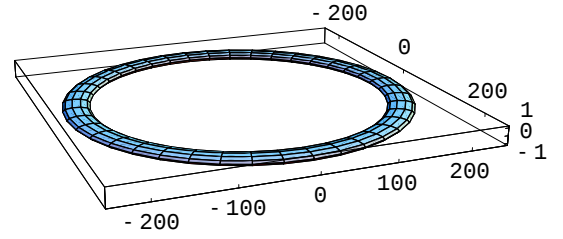
FIG. 2: (Color online) A view of the ring trap. An iso-potential surface is plotted for the parameters of Table I, in the harmonic approximation. The length unit is 1 \mu\text{m} . The vertical direction was amplified 10 times for clarity. The overall trap shape is that of a Saturnian ring.
