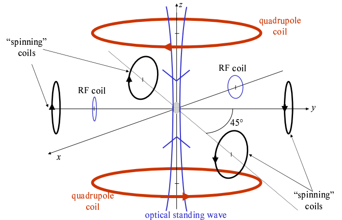
FIG. 4: (Color online) Coils and laser configuration for producing and exciting the ring trap. The trap is the combination of a vertical light standing wave (blue beam on the figure) and an egg shell rf trap (see section II). This egg shell trap relies on a magnetic field gradient (produced by the quadrupole coils) and rf coupling between Zeeman sub levels (two rf coils in quadrature as described in section VI). The additional “spinning” coils could be used for exciting the rotation of the atoms inside the ring trap (see section VII).
