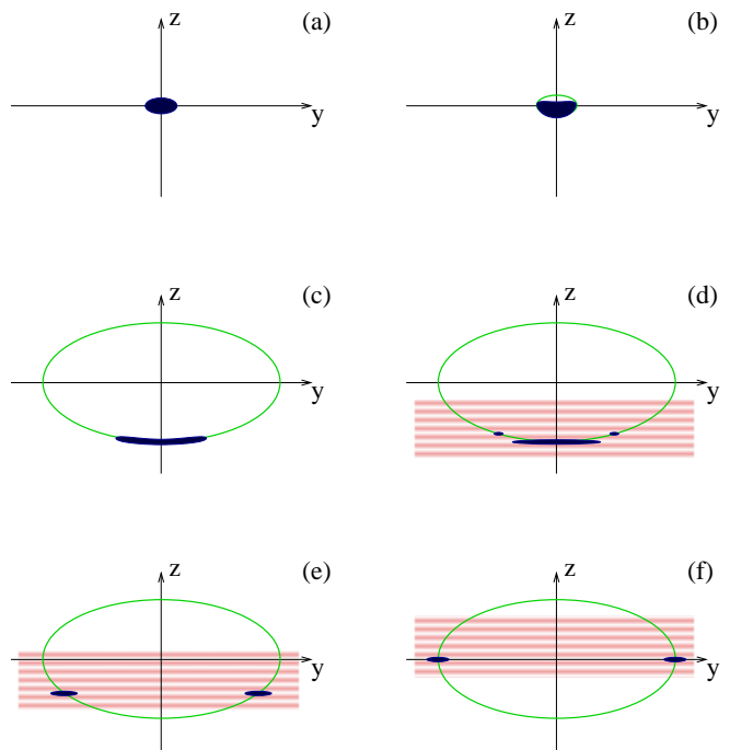
FIG. 3: (Color online) Outline illustration of stages in the loading of the ring trap. The z -axis is in the vertical direction and we assume a cylindrical symmetry about this axis. In (b-f) the elliptical line indicates the location (in the y - z plane) of the rf resonance. In (d-f) the grey bands indicate the presence of the standing light wave. Then: (a) We take as the starting point a BEC in a magnetic trap. (b) Shortly after transfer to the dressed rf trap the condensate fills a location around the rf resonance, but is not yet excluded from the trap centre. (c) After rf expansion (stage (ii)) the condensate lies at the bottom of the ‘egg-shell’. (d) The application of the optical standing wave results in a potential which confines the condensate to a couple of potential wells (corrugations). (e) The standing wave is moved upwards and the condensate ring is formed and expanded outwards and upwards. (f) Final position of the condensate ring at maximum radius. All three potentials, magnetic, dressed rf, and optical are required to maintain the ring.
