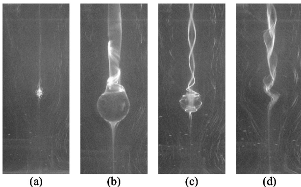
FIG. 4. Effect additional swirl by the small disk rotation on the breakdown bubble: (i) Re=1441 (a) \epsilon=0 and (b) corotation at \epsilon=0.72 , (ii) Re=1507 (c) \epsilon=0 and (d) counterrotation at \epsilon=-0.92 . Note: only the central region of the test section is shown.
