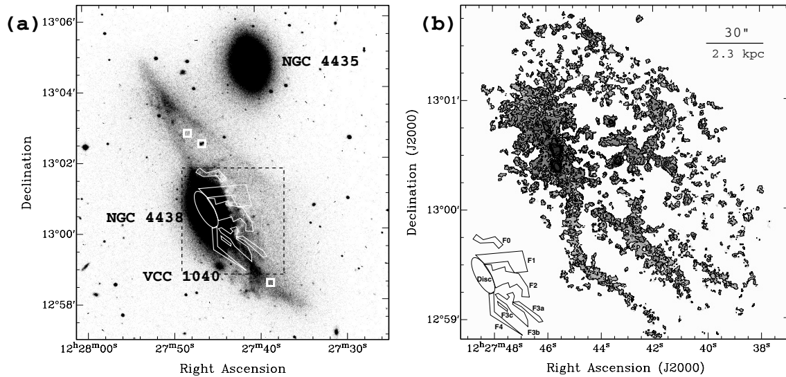
Fig. 1. a) A view of NGC 4435, NGC 4438 and VCC 1040. The optical map is a B -band image taken from the GoldMine database (Gavazzi et al. 2003). Contours display the approximate coverage of the total H\alpha emission. White squares correspond to the positions of selected spectra from the M é gantic FP observation (see Sect. 2.2, Table 3 and Fig. 6). The coordinates are in J2000. Notice the large dust layer on which the H\alpha emission superposes to the North and West of the disk of NGC 4438. A dashed box corresponds to the field of view seen in the right panel. b) Contours and grey-scale (displayed using a logarithmic stretch) map of the total integrated H\alpha emission. The first contour is at a higher intensity than the minimum level of the grey-scale image. The bottom-left, reduced-scale cartoon indicates the nomenclature used for the filaments.
