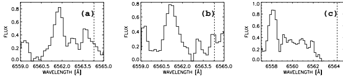
Fig. 6. Fabry-Perot continuum-free spectra of selected regions (see coordinates in Table 3 and white squares in Fig. 1). The spectra are averaged in a box of 8'' \times 8'' around centres of Table 3. The flux unit is arbitrary. The dashed lines indicate the systemic velocity of the galaxy.
