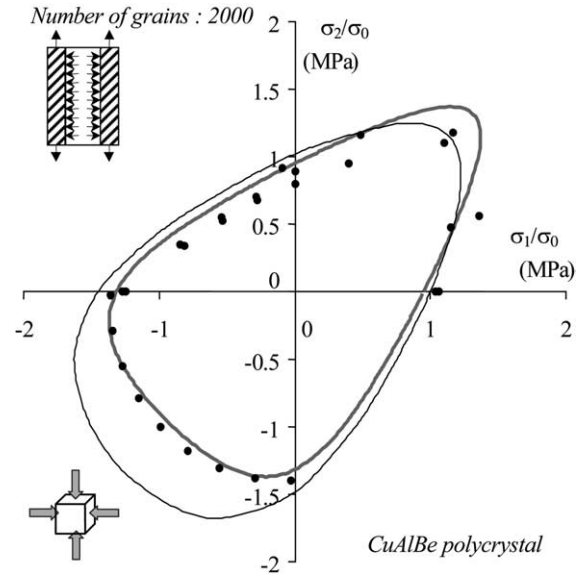
Fig. 3. Yield surface of Cu–Al–Be polycrystal in the space (\sigma_1, \sigma_2) (austenite → untwinned martensite) (● experimental points; — micro–macro simulation; - - phenomenological simulation).
