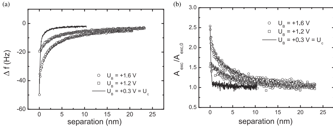
Figure 3. Frequency shift and ratio A_{\text{exc}}/A_{\text{exc},0} versus distance for different bias voltages recorded on Al(111). When applying +0.3 V on the sample, the contact potential is compensated and the electrostatic interaction is minimized. The electrostatic interaction adds a long-range component to both curves. A = 6.5 nm, f_0 = 162\,050 Hz, k_c = 29.4 N m ^{-1} , Q_0 = 31\,500 .
