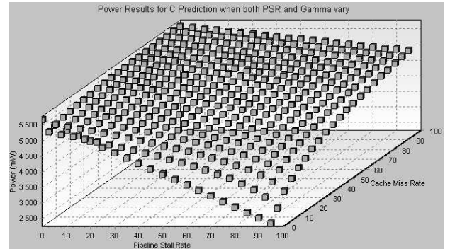
Fig. 1. C area: the power is a function of PSR and \gamma
