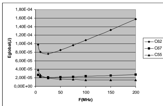
Fig. 6. Energy vs Frequency for the MPEG-1 decoder
