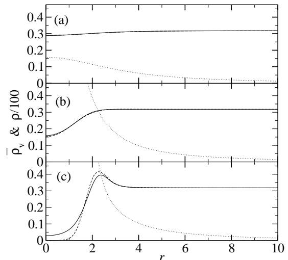
FIG. 2: Vortex ( \bar{\rho}_v ) and atomic ( \rho ) densities. Solid line: result for \bar{\rho}_v in the grand canonical ensemble. Dashed line: result for \bar{\rho}_v in the canonical ensemble with the same mean number of particles N . Dotted line: result for \rho/100 in the grand canonical ensemble. k_B T = 500 \epsilon_1 with \epsilon_1 = \hbar(\omega - \Omega) . (a) \mu = -10 \epsilon_1 ( N = 1986 ). (b) \mu = -\epsilon_1 ( N = 3396 ). (c) \mu = -0.1 \epsilon_1 ( N = 8320 ). The unit length is a_{ho} .
