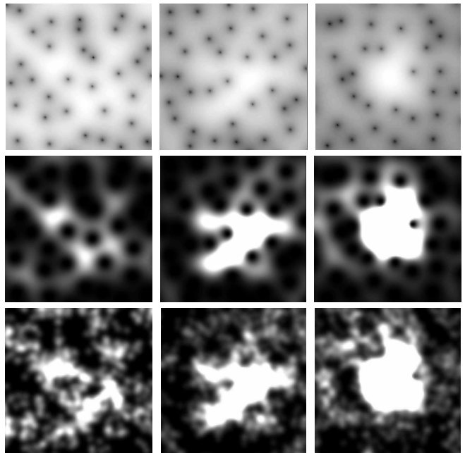
FIG. 1: Density plots for three randomly generated fields \psi , using the grand canonical ensemble for k_B T = 500 \epsilon_1 ( \epsilon_1 = \hbar(\omega - \Omega) ). Left column: \mu = -10 \epsilon_1 , mean number of particles N = 1986 ; middle column: \mu = -\epsilon_1 , N = 3396 ; right column: \mu = -0.1 \epsilon_1 , N = 8320 . First line: \ln(|\psi(\mathbf{r})|^2) . Second line: |\psi(\mathbf{r})|^2 . Third line: simulation of a real experiment; N random atomic positions are generated according to the density |\psi(\mathbf{r})|^2 , and a 129 \times 129 pixel ‘camera’ image is produced assuming that each atom produces a Gaussian spot of \sigma = 0.2a_{\text{ho}} . The width of each image is 10a_{\text{ho}} . Experimentally, a time of flight technique can be used to magnify these images, since the LLL modes are self-similar under a ballistic expansion.
