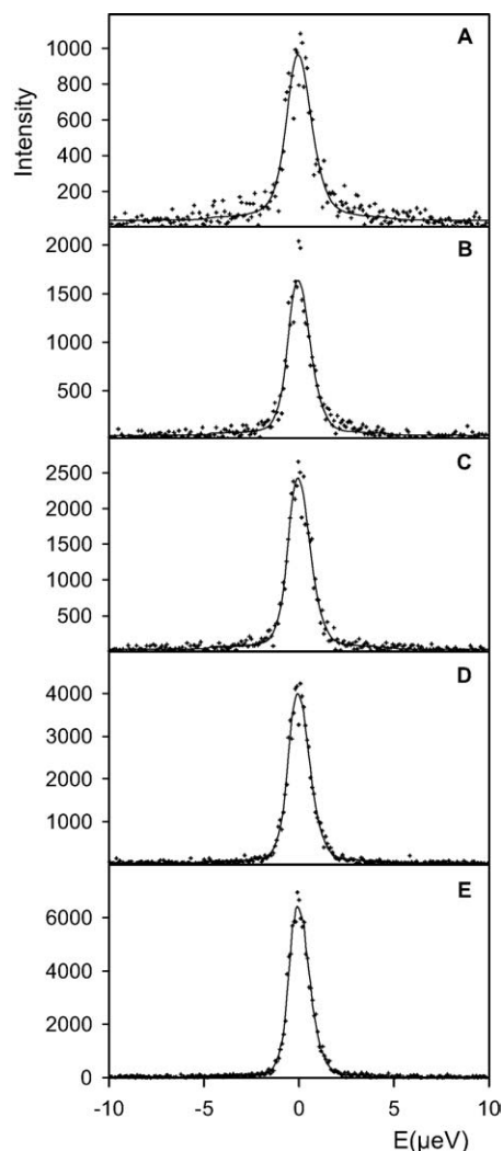
Fig. 1. Comparison between experimental (+) and calculated (solid lines) QENS spectra obtained for a concentration of 15 water molecules per supercell of BaX ( Q = 0.15 Å -1 ). The temperature of the sample was 440 \pm 1 K. Spectra were recorded from (a) to (e) (duration of one run: 4 h).
