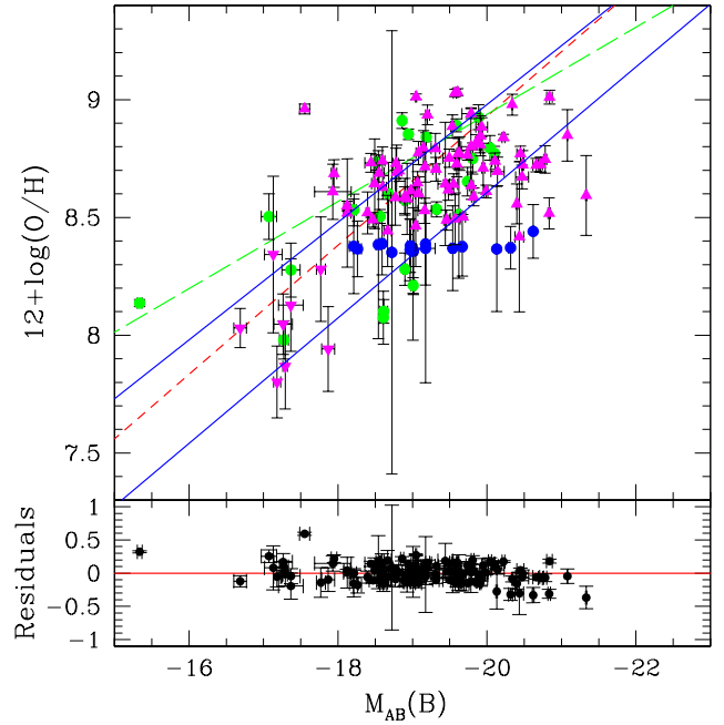
Figure 12. The “region-fitted” L-Z relations for our own sample of intermediate-redshift galaxies. The metallicities are derived with the R_{23} method. The solid lines represent the two linear regressions for the metal-poor and metal-rich galaxies (see text for details). Same legend as in Fig. 7 for the data points. The bottom panel shows the residuals around these two fits.
