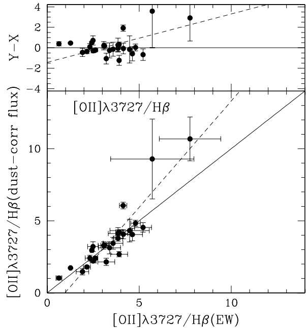
Figure 16. Comparison between the equivalent-width ( x -axis) and dust-corrected flux ( y -axis) ratio of [OII]\lambda 3727 and H\beta emission lines. The solid line shows the y = x curve and the dashed line is the fit to the data.
