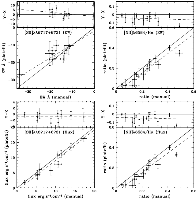
Figure 7. Comparison between blended features computed from equivalent width (in Å, top panels) and from fluxes (in 10^{-17} erg s^{-1} cm^{-2} , bottom panels) automatically (using platefit ) and manually (using IRAF task splot ): the line sum [SII] \lambda\lambda 6717+6731 (left) and the line ratio [NII] \lambda 6584/H \alpha (right). The solid line is the x = y line and the dashed line is the linear regression.
