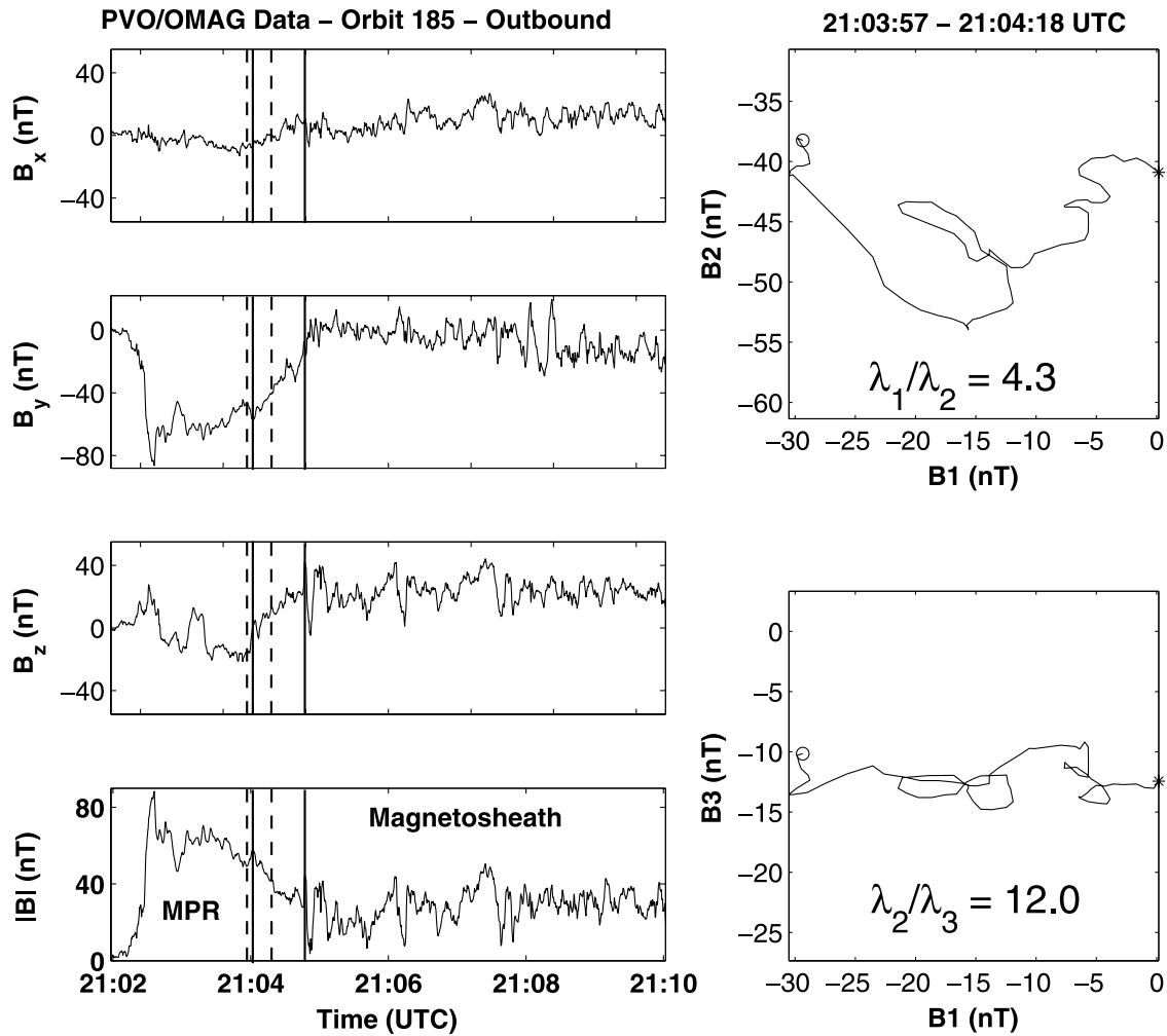
Figure 4. High-resolution ( 4 \text{ s}^{-1} ) PVO/OMAG data (VSO coordinates) around a Venusan MPB crossing (solid lines) on orbit 185 around 17^\circ SZA. MVA is applied between 2103:57 and 2104:18 UTC (dashed lines). On the right, hodograms show the magnetic field components on the minimum variance planes ( \mathbf{e}_1, \mathbf{e}_2 ) and ( \mathbf{e}_1, \mathbf{e}_3 ). Start and the end of the hodograms are marked with circles and stars, respectively. Eigenvalue ratios are also indicated.
