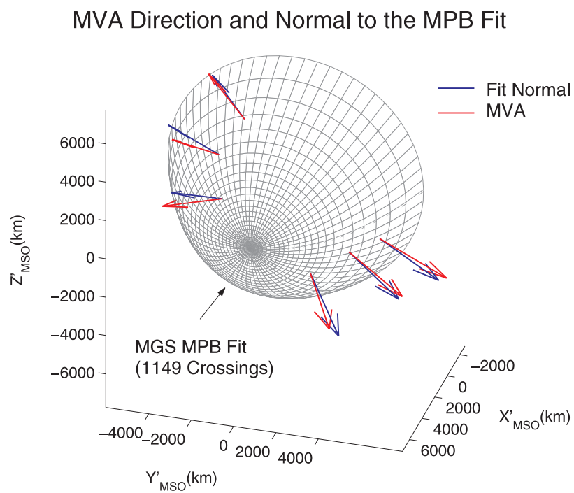
Figure 3. Comparison between minimum variance direction and the normal expected from a MPB ellipsoid fit from 1149 Martian MGS crossings based on Vignes et al. [2000] work (blue arrows). Sketch is represented in 4^\circ -aberrated MSO coordinates.
