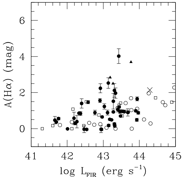
Fig. 1. (a) The extinction in the H \alpha line, A(H \alpha ), as measured with the Balmer decrement versus the FIR luminosity. The SFG sample is plotted with filled circles, the 3 lower limits in A(H \alpha ) are plotted with triangles. The errors on A(H \alpha ) are also plotted. The IUE sample is plotted with empty symbols: circles for the galaxies with d_{25} < 1.5 arcmin and squares for the larger ones. M82 is plotted as a cross.
