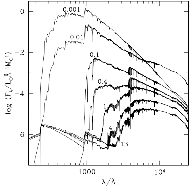
Figure 9. Spectral evolution of the standard SSP model of Section 3 for the solar metallicity. The STELIB/BaSeL 3.1 spectra have been extended blueward of 3200 Å and redward of 9500 Å using the Pickles medium-resolution library. Ages are indicated next to the spectra (in Gyr).
