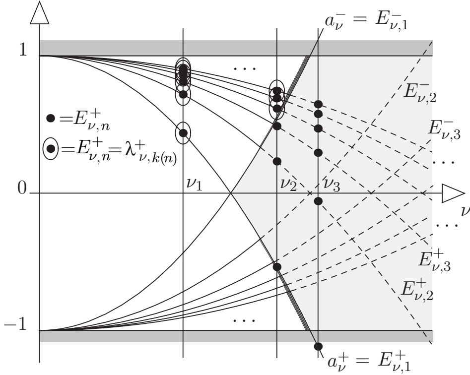
Figure 1: Depending on the values of \nu , all eigenvalues are achieved by the two families of levels \lambda_{\nu,k}^+ and \lambda_{\nu,k}^- (Case \nu = \nu_1 < 2 ), or only some of them (Case \nu = \nu_2 \in (2, \sqrt{8}) ). For \nu > \sqrt{8} (Case \nu = \nu_3 ), the gap (-1, 1) is contained in (a^+, a^-) and the method does not characterize any eigenvalue in the gap. To clarify the picture, only the family of eigenvalues E_{\nu,n}^+ has been represented, but the family E_{\nu,n}^- is easily recovered by symmetry with respect to the horizontal axis. To take the multiplicity into account, we denote by k(n) the smallest k for which \lambda_{\nu,k}^+ = E_{\nu,n}^+ .
