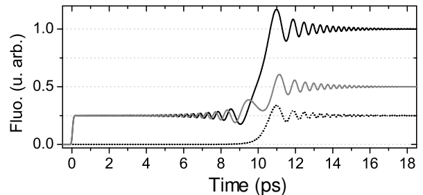
FIG. 1: Simulation of Coherent Transients resulting from the excitation of the atom by a FT limited pulse (at time t=0 ) followed by a chirped pulse (centered at t=10\text{ps} ). For \theta = 0 (black) and \theta = \pi/2 (gray). Dotted line: "Simple" CTs obtained for a single pulse at t=10\text{ps} .
