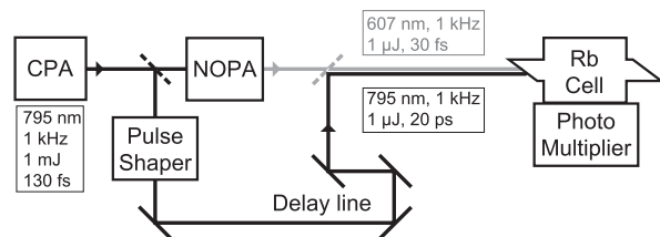
FIG. 2: Experimental set-up. NOPA : non collinear optical parametric amplifier; CPA: Chirped Pulse Amplifier
