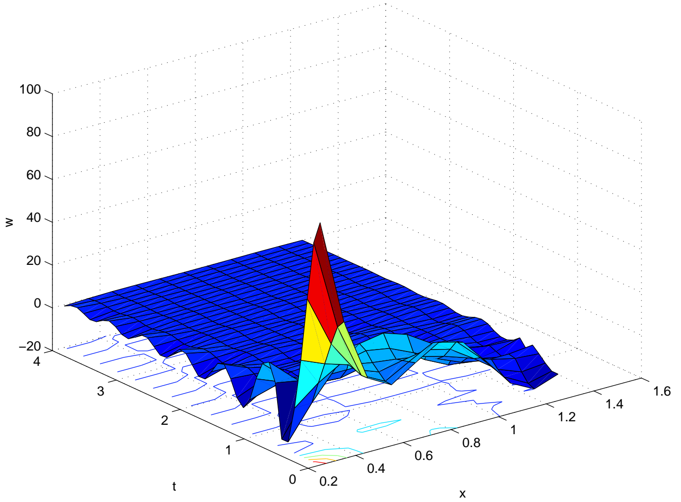
approximate solution
