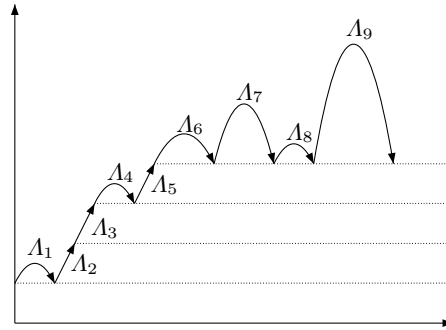
Fig. 2. P/B Factorization
