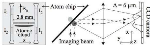
FIG. 1: Schematic of the experimental setup. Left: drawing of the wires constituting the atom chip. We keep I_1 + I_2 = 3 A and adjust I_1 - I_2 between 0.3 A and 1 A to vary the confinement along z . The uniform field B_0 is approximately 40 G, we also add a small field ( \lesssim 1 G) along z . Right: optical imaging system. We image the cloud and its reflection on the atom chip onto a CCD camera. In the radial direction, the unresolved cloud images cover approximately five pixels whose size in the object plane is \Delta = 6 \mu\text{m} .
