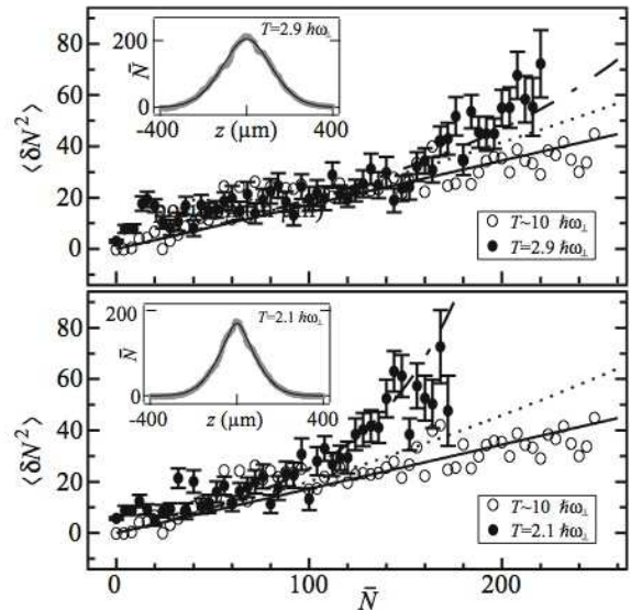
FIG. 2: Atom number variance as a function of the mean atom number per pixel. Open circles correspond to a "hot" cloud ( k_B T \simeq 10 \hbar \omega_\perp , \omega_\perp = 2\pi \times 2.85 kHz) for which fluctuations are given by the shot noise (black line). The full circles correspond to cold clouds. Error bars show the standard deviation of the mean of \langle \delta N^2 \rangle . The fluctuations in excess of shot noise are due to bosonic bunching. The dot-dashed line is the prediction for an ideal Bose gas while the dotted line uses the Maxwell-Boltzmann approximation (see Eq. (3)). The insets show the longitudinal profile of the two cold clouds from which we deduce the temperature and the chemical potential used for the calculations.
