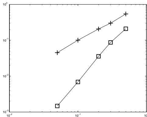
Figure 1: p = 1.5 . Relative errors \frac{\|u - \bar{u}\|_p}{\|\bar{u}\|_p} (“□”; slope \approx 2.1 ) and \frac{\|\mathbf{v} - \nabla \bar{u}\|_p}{\|\nabla \bar{u}\|_p} (“+”; slope \approx 1 ) versus the size of the discretization, in log-log scale.
