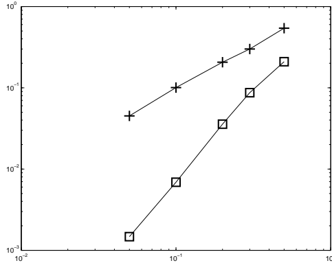
Figure 1: p = 1.5 . Relative errors \frac{\|u - \bar{u}\|_p}{\|\bar{u}\|_p} (“□”; slope \approx 2.1 ) and \frac{\|\mathbf{v} - \nabla \bar{u}\|_p}{\|\nabla \bar{u}\|_p} (“+”; slope \approx 1 ) versus the size of the discretization, in log-log scale.
