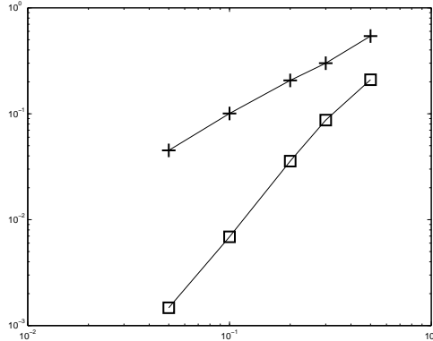
Figure 1: p = 1.5 . Relative errors \frac{\|u-\bar{u}\|_p}{\|\bar{u}\|_p} (“ \square ”; slope \approx 2.1 ) and \frac{\|\mathbf{v}-\nabla\bar{u}\|_p}{\|\nabla\bar{u}\|_p} (“ + ”; slope \approx 1 ) versus the size of the discretization, in log-log scale.
