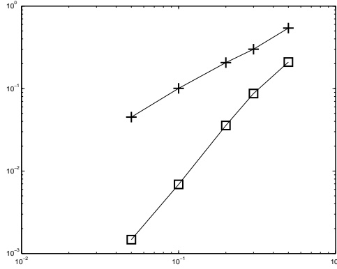
Figure 1: p = 1.5 . Relative errors \frac{\|u-\bar{u}\|_p}{\|\bar{u}\|_p} (“ \square ”; slope \approx 2.1 ) and \frac{\|\mathbf{v}-\nabla\bar{u}\|_p}{\|\nabla\bar{u}\|_p} (“+”; slope \approx 1 ) versus the size of the discretization, in log-log scale.
