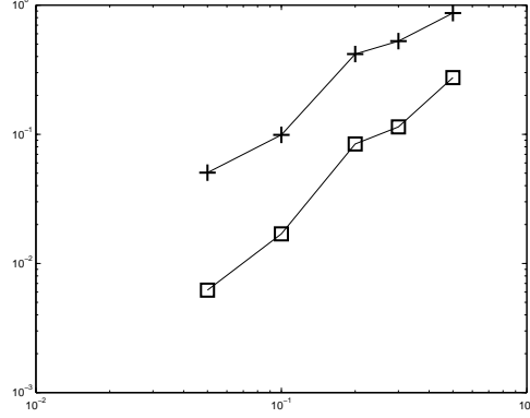
Figure 2: p = 4 . Relative errors \frac{\|u-\bar{u}\|_p}{\|\bar{u}\|_p} (“□”; slope \approx 1.6 ) and \frac{\|v-\nabla\bar{u}\|_p}{\|\nabla\bar{u}\|_p} (“+”; slope \approx 1.2 ) versus the size of the discretization, in log-log scale.
